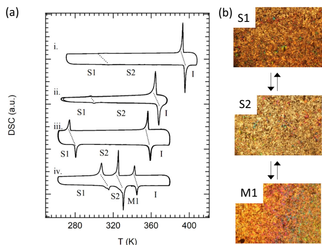
Fig. 4 Phase-transition behavior of C n SS derivatives ( n = 6, 8, 10, \text{ or } 16 ). a DSC curves of (i) C6SS , (ii) C8SS , (iii) C10SS , and (iv) C16SS , where transformations between the S1, S2, and M1 phases were reversible in the T -cycle. b POM images of C16SS at S1 ( T = 300 \text{ K} ), S2 ( T = 320 \text{ K} ), and M1 ( T = 330 \text{ K} ).
