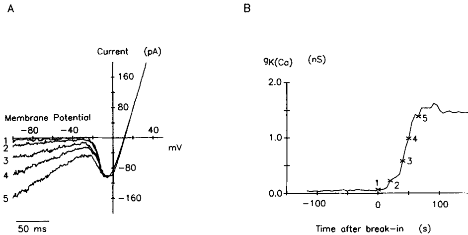
FIGURE 3. Induction of I_{1(\text{Ca})} by whole-cell dialysis with 10 \mu\text{M} free \text{Ca}^{2+} . (A) Ramp currents obtained 1, 20, 30, 35, and 45 s after establishing whole-cell recording mode (traces 1–5, respectively). A progressive increase in I_{1(\text{Ca})} induced by the pipette \text{Ca}^{2+} is manifest as the increase in slope conductance at potentials below -30 mV. Internal solution: K aspartate + 10^{-5} M \text{Ca}^{2+} . External solution: K + Ringer. This internal solution is also used to induce I_{1(\text{Ca})} in the experiments shown in Figs. 4–7. (B) K(Ca) conductance measured from the experiment shown in A, plotted as a function of time after attaining whole-cell configuration (“break-in”). The numbered points correspond to the current traces shown in A.
