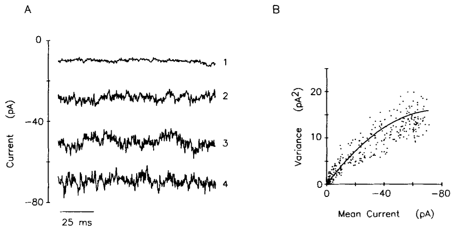
FIGURE 9. Fluctuation analysis of the apamin-sensitive K(Ca) current in the whole-cell recording mode. I_{1(\text{Ca})} was induced by intracellular dialysis with 1 \mu\text{M} \text{Ca}^{2+} , with 20 nM CTX added to the K + Ringer external solution to block voltage-gated K + channels (Fig. 4) and the larger, CTX-sensitive K(Ca) channels present in these cells (Fig. 7). (A) Currents recorded at -80 mV during induction of K(Ca) during dialysis with a pipette solution containing 1 \mu\text{M} \text{Ca}^{2+} . As I_{1(\text{Ca})} develops, the holding current amplitude progressively increases (traces 2-4). Note the changes in current fluctuations as the mean current level is increased. Trace 1 was recorded before the induction of I_{1(\text{Ca})} and gives a measure of leak current and background variance. (B) Current variance plotted as a function of mean current for the experiment in A. Each point represents the variance and mean of a single 110-ms trace. Variance was obtained by averaging the square of the fluctuations around the mean current level. A parabola of the form:
