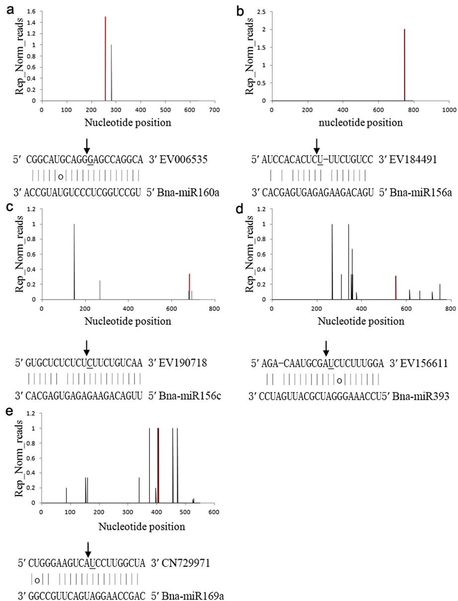
Figure 3 Confirmed microRNA (miRNA) targets using degradome sequencing are presented in the form of target plots (t-plots). We used normalized numbers in plotting the cleavages on target mRNAs, which were referred to as 'target plots' (t-plots) by German et al. [51]. Signature abundance throughout the length of the indicated transcripts is shown. Representative t-plots for class 0 (a), class I (b), class II (c), class III (d), and class VI (e) categories are shown. Arrows indicate signatures consistent with miRNA-directed cleavage. miRNA:mRNA alignments along with the detected cleavage frequencies (normalized numbers) are shown. The frequencies of degradome tags with 5'ends at the indicated positions are shown in black, with the frequency at position 10 of the inset miRNA target alignment highlighted in red. The underlined nucleotide on the target transcript indicates the cleavage site detected in the degradome.
