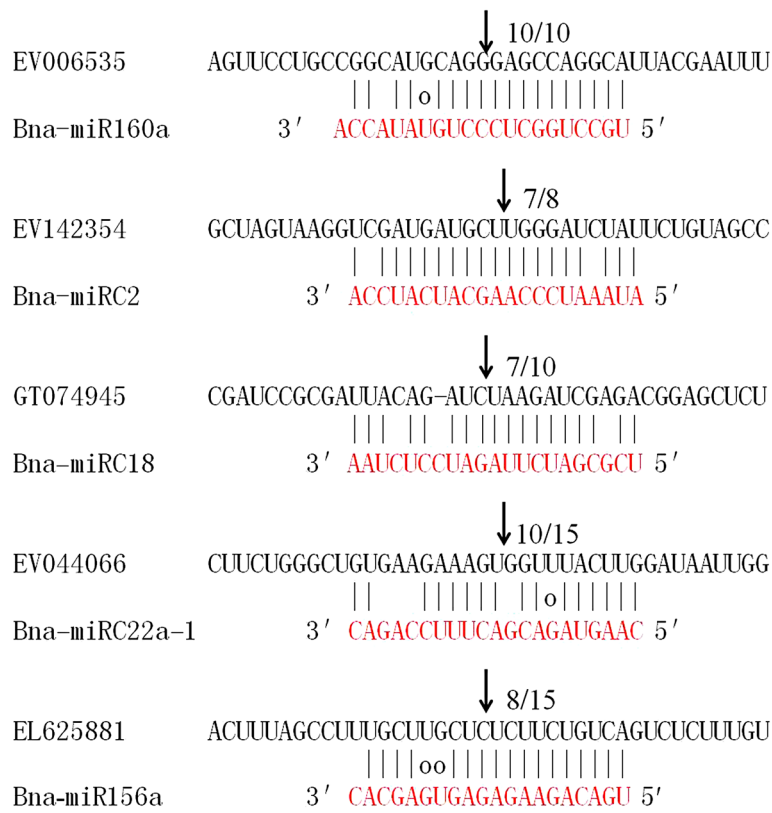
Figure 4 Mapping of the mRNA cleavage sites by RNA ligase-mediated 5'RACE. Each top strand (black) depicts a miRNA complementary site, and each bottom strand depicts the miRNA (red). Watson-Crick pairing (vertical dashes) and G:U wobble pairing (circles) are indicated. The arrows indicate the 5' termini of mRNA fragments isolated from B. napus , as identified by cloned 5' RACE products, with the frequency of clones with the predicted cleavage site shown.
