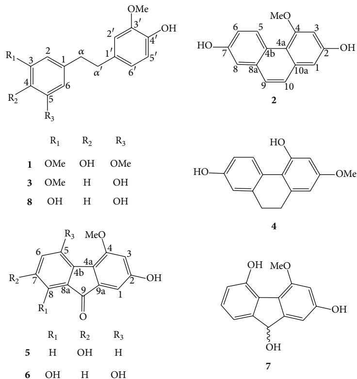
FIGURE 1: Structures of compounds 1–8 from Dendrobium brymerianum .
