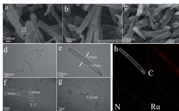
Fig. 3 (a and b) SEM image of CNT and carbonized CNT; (c–h) SEM, TEM, HRTEM and HAADF-STEM of Ru@CNT-500 and corresponding EDS element map. ((c) is SEM; (d and e) is TEM; (f and g) is HRTEM, and (h) is HAADF-STEM and STEM-EDS diagram).
