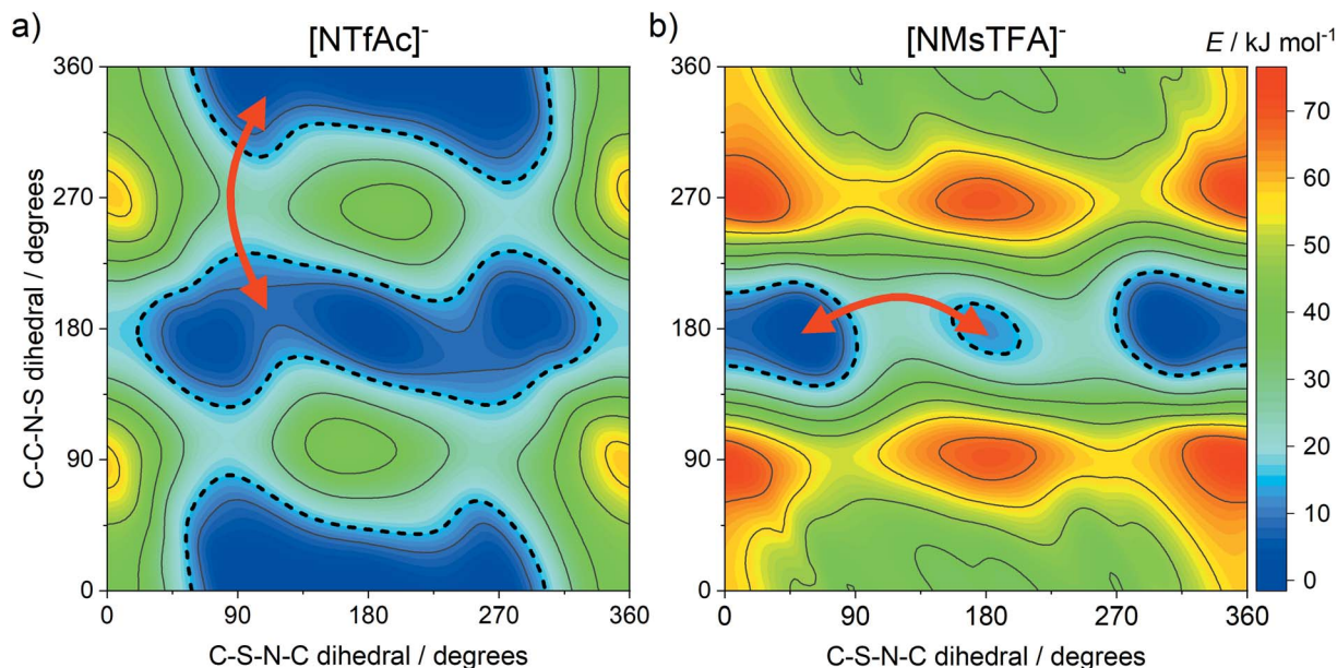
Fig. 8 Potential energy surfaces of (a) [\text{NTfAc}]^- and (b) [\text{NMStFA}]^- , red arrows indicate plausible transitions between basins in line with the DMTA measurements.
