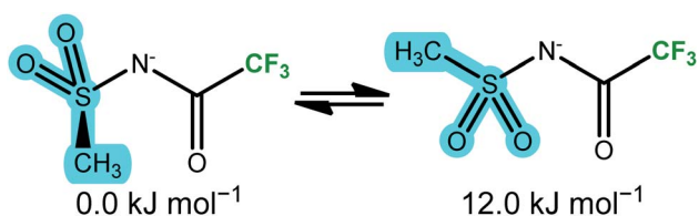
Fig. 9 The two unique minimum energy geometries in [\text{NMStFA}]^- , cf. Fig. 8b.
