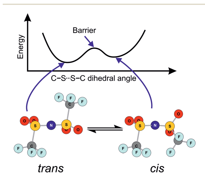
Fig. 1 Schematic of the two minimum energy conformers of the [NTf 2 ] − anion, and of the energy as a function of the C–S...S–C dihedral angle. Adapted from ref. 39.
