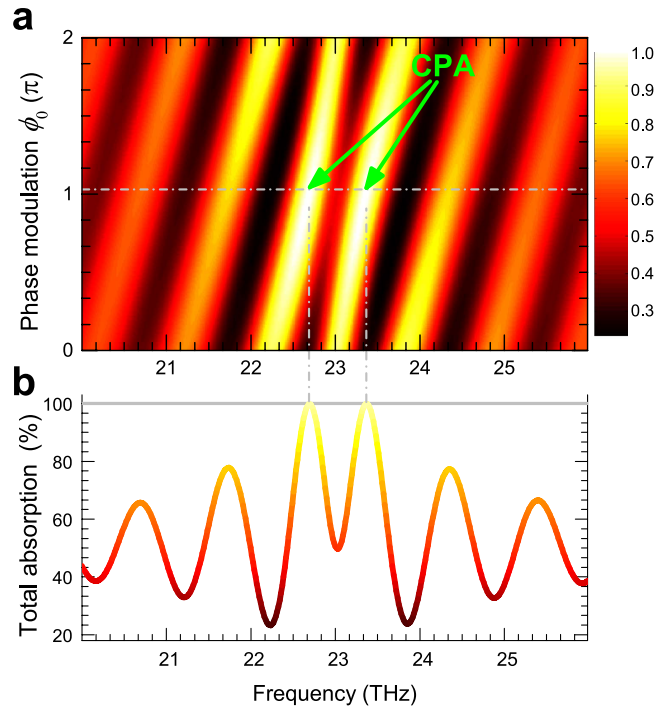
Figure 3. A two-dimensional false-color plot of the normalized total absorptions as a function of frequency and phase modulation \phi_0 , the exact CPA points are denoted with green arrows.
