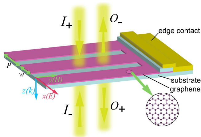
Figure 1. Schematic of a graphene ribbon meta-surface illustrated by two counter-propagating and coherently modulated input beams ( I_+ and I_- , the electric polarization is along x -axis, and propagate along \pm z -directions), O_+ and O_- represent the amplitudes of output beams.
