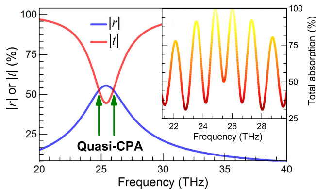
Figure 6. Scattering coefficients of a graphene nanoribbon array with experimental data (Yan et al. data), the inset shows normalized total absorption for proper phase modulation.
