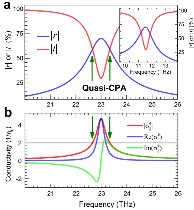
Figure 2. (a) Spectra of the reflection and transmission coefficients of a graphene nanoribbon meta-surface ( w = 0.33 \mu\text{m} ), the quasi-CPA points at the crosses of the scattering spectra are indicated with arrows. (b) Absolute values, real and imaginary parts of the effective surface conductivities of the corresponding graphene nanoribbon meta-surface.
