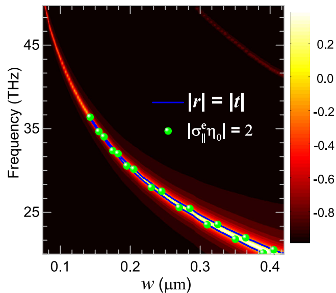
Figure 4. Geometric tunability of the graphene meta-surface CPA: Spectra of the difference ( |r| - |t| ) of the scattering coefficients ( r and t ) for the graphene meta-surface width increasing from 0.075 \mu\text{m} to 0.42 \mu\text{m} . The solid line indicates quasi-CPA points where |r| = |t| , while the spheres represent the extracted surface conductivities with values |\sigma_{||}^e| \eta_0 = 2 .
