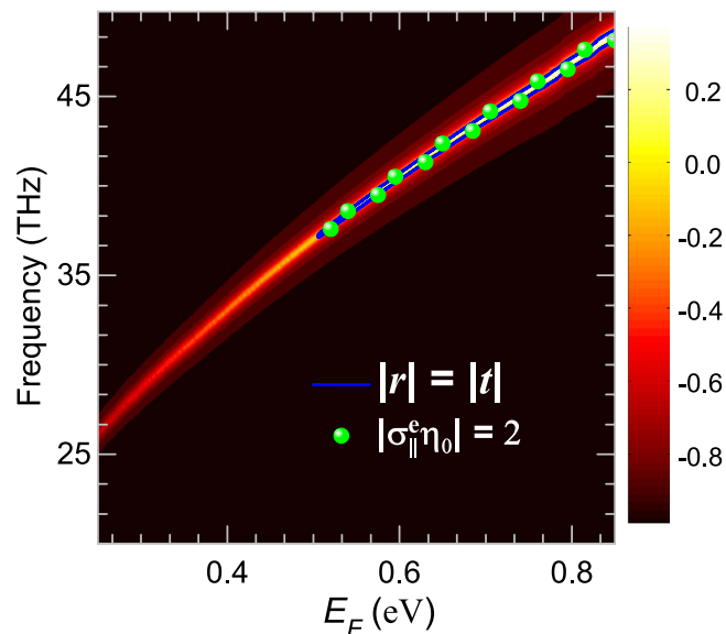
Figure 5. Electric tunability of the graphene meta-surface CPA: Spectra of the difference ( |r| - |t| ) of the scattering coefficients ( r and t ) for the graphene meta-surface with Fermi energy E_F ranging from 0.25 \text{ eV} to 0.85 \text{ eV} . The solid line indicates quasi-CPA points where |r| = |t| , while the spheres represent the extracted surface conductivities with values |\sigma_{||}^e| \eta_0 = 2 .
