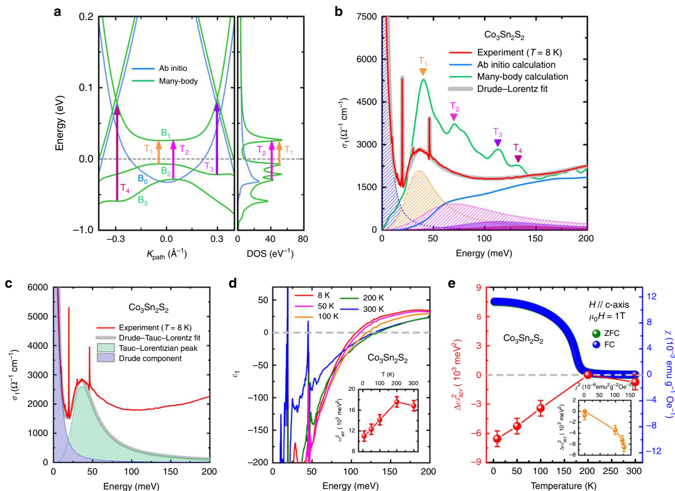
Fig. 4 Flat band and related optical transitions in ferromagnetic \text{Co}_3\text{Sn}_2\text{S}_2 . a Left panel: quasiparticle band structure obtained by many-body calculations (i.e., DFT + DMFT calculations) (green curve) and band structure gotten by single-particle ab initio calculations in the FM ground state (blue curve) along the direction connecting the Weyl points. Right panel: density of states (DOS) of the quasiparticle bands. The four arrows in the left panel show the optical transitions related to the flat band B_1 or the dispersionless part of band B_2 (or B_3 ) with divergent DOS. b Experimental and calculated real parts \sigma_1(\omega) of the optical conductivity at low energies. Four peak-like features ( T_1 , T_2 , T_3 , and T_4 ) in the \sigma_1(\omega) obtained by many-body calculations are present around 38, 70, 113, and 131 meV, respectively. These four peak-like features arise mainly from the four optical transitions illustrated by the four arrows in a . The asymmetric peak-like feature around 36 meV in the experimental \sigma_1(\omega) at T = 8 K can be fitted with the four Lorentzian peaks (see the shaded peaks in b ), which are located around 36, 70, 113, and 131 meV, respectively. Peak-like feature is absent around 38 meV in the interband-transition-contributed part of the \sigma_1^T(\omega) obtained by single-particle ab initio calculations in the FM ground state (see the blue spectrum in b ). c Drude-Tauc-Lorentz fit to the experimental \sigma_1^E(\omega, T = 8 K) of \text{Co}_3\text{Sn}_2\text{S}_2 . The green and blue shaded areas are the Tauc-Lorentzian peak and the Drude component, respectively. The gray curve shows the Drude-Tauc-Lorentz fit to the experimental peak-like feature around 36 meV in the \sigma_1^E(\omega, T = 8 K). d Real parts \epsilon_1(\omega) of the dielectric functions of \text{Co}_3\text{Sn}_2\text{S}_2 at different temperatures. The inset in d shows the squares \omega_{\text{scr}}^2 of its screened plasma frequencies at different temperatures. e Relative squares of the screened plasma frequency \Delta\omega_{\text{scr}}^2 = \omega_{\text{scr}}^2(T) - \omega_{\text{scr}}^2(T = 200 K) at different temperatures (see red dots) and temperature dependence of the magnetic susceptibility \chi with zero-field-cool (ZFC) and field-cool (FC) modes in a magnetic field B = 1 T for B//c -axis (see green and blue dots). In e the ZFC-mode susceptibility data are covered by the FC-mode susceptibility data 52 . The inset of e displays the \chi^2 dependence of the \Delta\omega_{\text{scr}}^2 . The error bars on the data in d and e are based on the line thickness of the \epsilon_1(\omega) in d .
