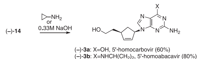
Scheme 4. Synthesis of target carbonucleosides ( - )- 3b and ( - )- 3a .
