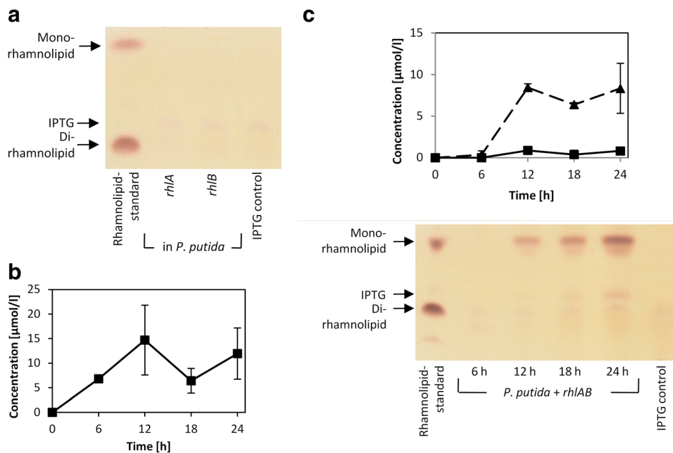
Fig. 2 Rhamnolipids and HAAs produced by recombinant P. putida . a Thin layer chromatography (TLC) of extracts from single rhlA or rhlB expression shows no detectable amounts of rhamnolipids after 24 h (HPLC results not shown). b HPLC analysis of HAAs reveals their production in a rhlA expressing P. putida strain. c HPLC analysis of HAAs (squares) and mono-rhamnolipids (triangles) and TLC of P. putida
