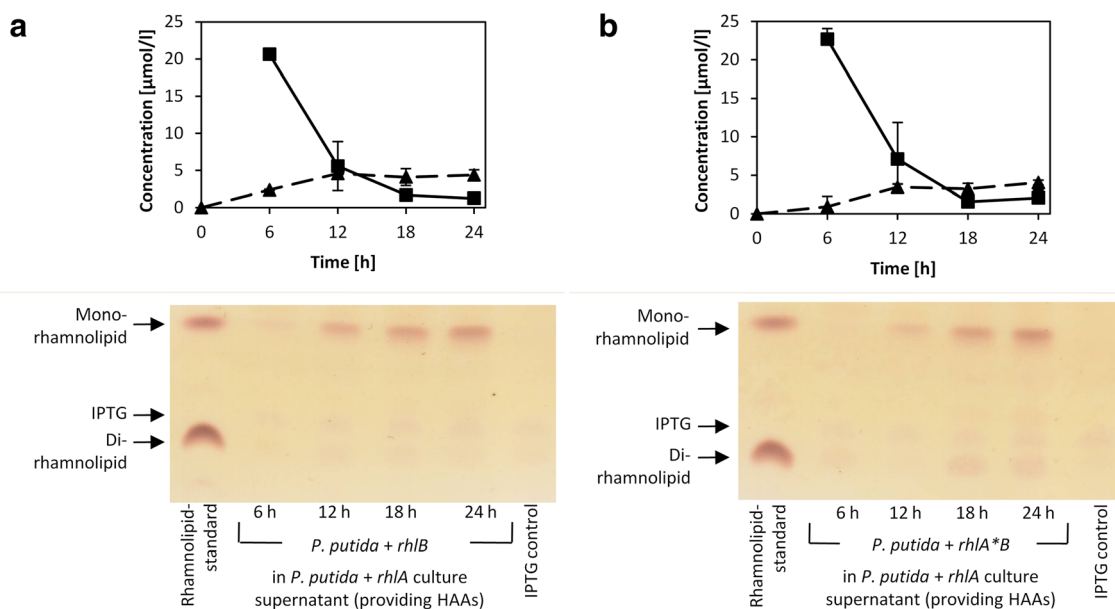
Fig. 4 Production of mono-rhamnolipids by recombinant P. putida in HAA containing conditioned medium. P. putida strains expressing single rhIB (a) or the rhIA*B operon (b), containing inactive RhIA, were cultivated in HAA containing conditioned medium, obtained from a rhIA expressing P. putida strain. Extracts were analyzed via HPLC revealing HAAs (squares) and mono-rhamnolipids (triangles) and thin
