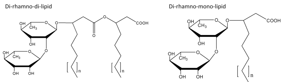
Fig. 1 Chemical structures of rhamnolipids. Rhamnolipids are separated into mono- and di-rhamnolipids based on the number of L-rhamnose residues. Beside typical rhamnolipid species containing two 3-hydroxyfatty acids (mono-rhamno-di-lipid and di-rhamno-di-lipid), there exist species containing only one fatty acid chain (mono-rhamno-mono-
