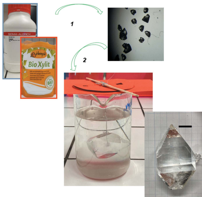
Figure 4 Growing large xylitol crystals. (1) Preparation of seed crystal. A seed crystal, glued to the end of a cotton thread, is placed in an aqueous saturated xylitol solution (~170 g of xylitol dissolved in 100 mL of water). (2) After several weeks, a large single crystal is obtained. The scale bar represents 10 mm.
