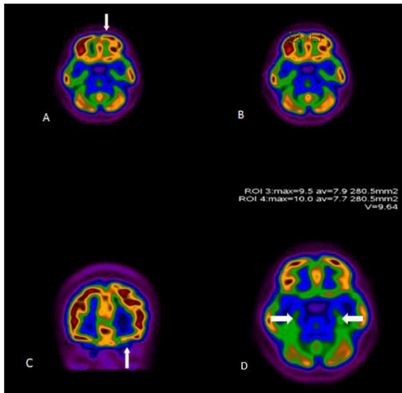
Figure 3 FDG-PET/CT scan of a 27-year-old woman with persistent anosmia and positive PCR for SARS-CoV-2. Representative axial (A, B, D) and coronal (C) images are shown. There was decreased uptake in the left orbitofrontal cortex (arrows). The uptake of temporal lobes were symmetric and normal (arrows, D). Figure 3 reproduced with permission from Karimi-Galougahi M, Yousefi-Koma A, Bakhshayeshkaram M, Raad N, Haseli S. 18FDG PET/CT scan reveals hypoactive orbitofrontal cortex in anosmia of COVID-19. Academic radiology 2020; 27:1042-1043.
