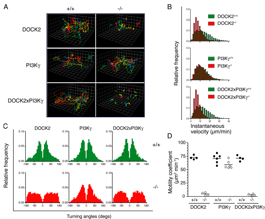
Figure 1. Paracortical T cell migration in the absence of DOCK2 and PI3K \gamma . Fluorescently labeled control T cells and DOCK2 -/- , PI3K \gamma -/- , or DOCK2 -/- \times PI3K \gamma -/- T cells were adoptively transferred into wild-type recipients, and their migratory behavior inside popliteal lymph nodes was analyzed using MP-IVM. The grid length of each square corresponds to 20.8 \mu\text{m} . (A) Representative three-dimensional tracks of control T cells (+/+; left column) and DOCK2 -/- , PI3K \gamma -/- , or DOCK2 -/- \times PI3K \gamma -/- T cells (-/-; right column) over 30-min periods. Each colored line represents a single T cell track. (B) Velocity profiles of control T cells (green bars) and DOCK2 -/- , PI3K \gamma -/- , or DOCK2 -/- \times PI3K \gamma -/- T cells (red bars).
