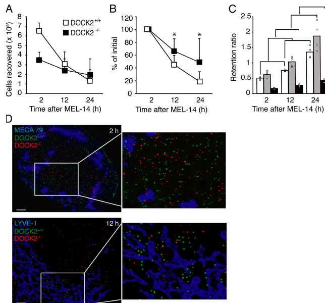
Figure 4. DOCK2 deficiency delays lymphocyte egress from PLNs.
