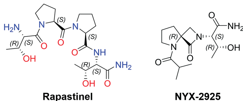
Figure 1. Structural comparison of the peptide rapastinel with the spirocyclic \beta -lactam, ((2 S , 3 R )-3-hydroxy-2-(( R )-5-isobutyryl-1-oxo-2,5-diazaspiro[3.4]octan-2-yl)butanamide) (NYX-2925). Spirocyclic \beta -lactam chemistry has been used to create a number of new molecules that mimic key properties of their parent peptides (Bittermann and Gmeiner, 2006).
