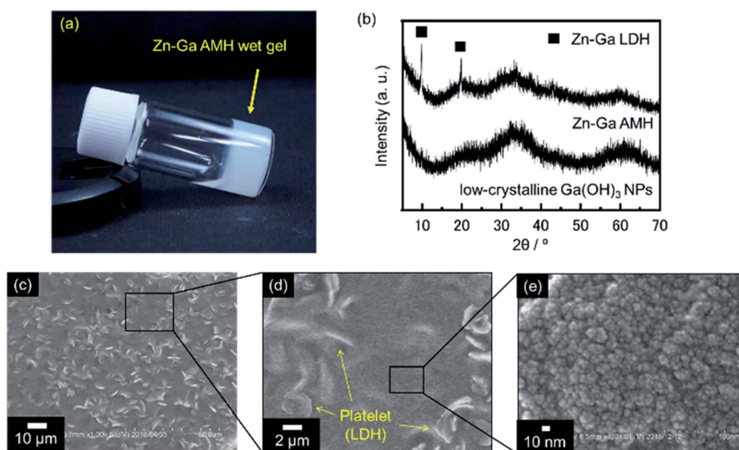
Fig. 1 (a) Photograph of precursory wet gel obtained from an aqueous solution of \text{Zn}(\text{NO}_3)_2 \cdot 6\text{H}_2\text{O} and \text{Ga}(\text{NO}_3)_3 \cdot n\text{H}_2\text{O} under a highly supersaturated condition induced by epoxide-mediated alkalization. (b) PXRD patterns of precursory xerogel and low-crystalline \text{Ga}(\text{OH})_3 NPs obtained from an aqueous solution of \text{Ga}(\text{NO}_3)_3 \cdot n\text{H}_2\text{O} (without \text{Zn}(\text{NO}_3)_2 \cdot 6\text{H}_2\text{O} ). (c–e) SEM images of precursory xerogel at different magnifications.
