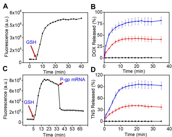
Fig. 3 (A) Release profile of DOX from the \text{MnO}_2\text{@TNS/DOX} nanoswitch triggered by 1 mM GSH. (B) Release profiles of DOX at GSH concentrations of 0, 0.6, and 1.0 mM. (C) Release profile of TNS from nanoswitch triggered by 1 mM GSH and activated by 400 nM P-gp mRNA. (D) Release profiles of TNS at different concentrations of GSH (0, 0.6, and 1.0 mM).
