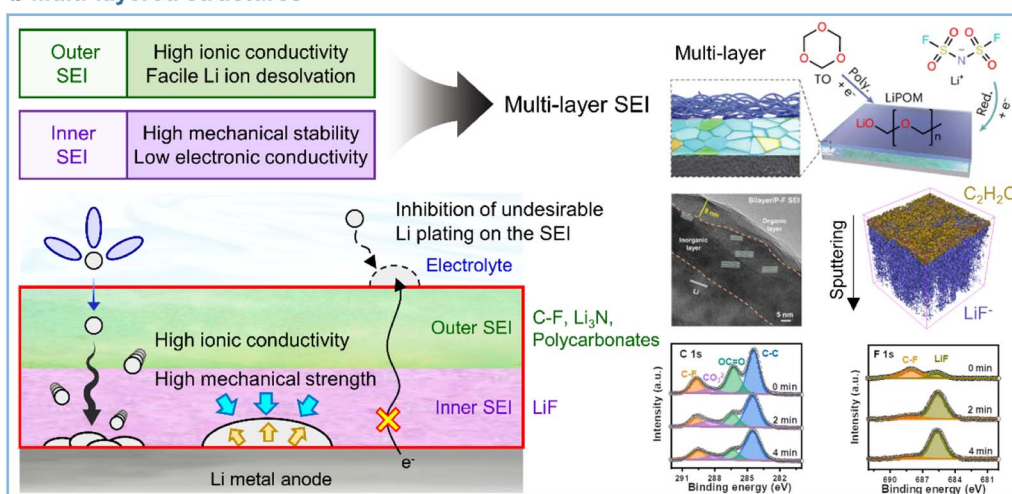
Fig. 9 Representative models for (a) lithiophilic materials and self-healing mechanisms and (b) multi-layered SEI structures. Reproduced from ref. 136, 137, and 138 with permission of American Chemical Society, copyright 2013, John Wiley & Sons, Inc., copyright 2021, and Springer Nature, copyright 2023, respectively.
