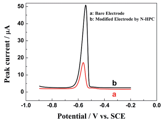
Fig. 4 The DPASV curves of the bare GCE (a) and N-HPC/GCE (b) in a 0.1 \text{ M HAC-NaAc} buffer solution at \text{pH } 5.0 containing 5.0 \mu\text{M Pb}^{2+} . Deposition potential: -0.8 \text{ V} ; amplitude: 50 \text{ mV} ; potential step: 4 \text{ mV} ; deposition time: 350 \text{ s} ; pulse period: 0.2 \text{ s} ; pulse width: 50 \text{ m s} ; sample width: 0.0167 \text{ s} ; and quiet time: 2 \text{ s} .
