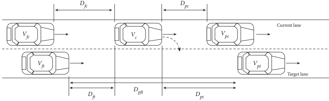
FIGURE 3: The typical lane-change scenario.
