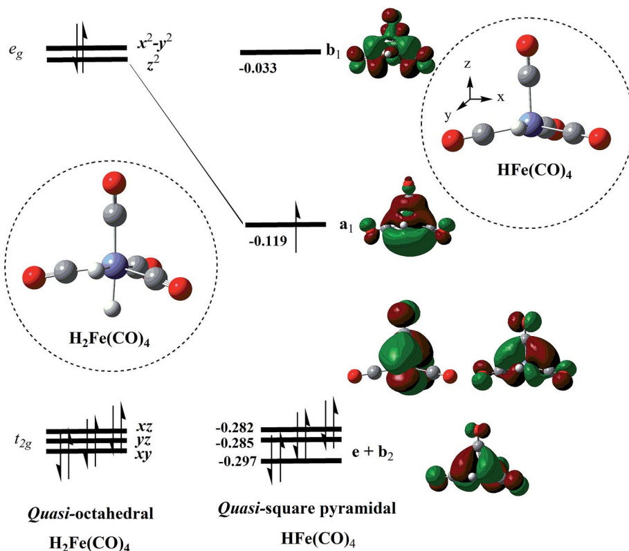
Fig. 4 Orbital diagram demonstrating the formation of the low-spin d^7 -isobal fragment-radical HFe(CO) 4 via the removal of the axial H-ligand from the quasi-octahedral precursor H 2 Fe(CO) 4 . The hybrid orbital a_1 in the HFe(CO) 4 radical is pointed toward the vacant octahedral vortex. The orbital energies are in eV and were calculated at the ROB3LYP/BS-I level.
