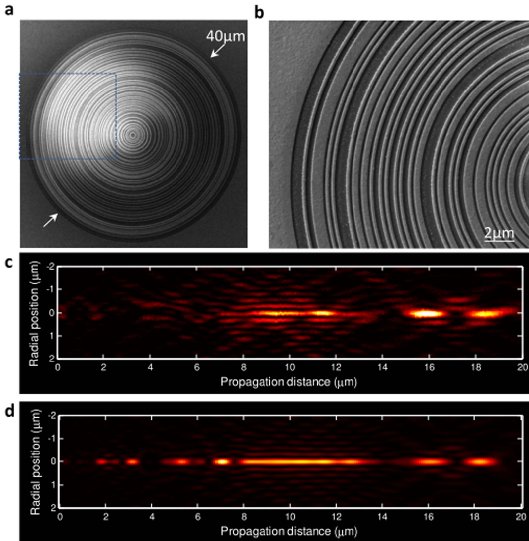
Figure 1 | SOL design and diffraction patterns in longitudinal cross-section. (a), SEM image of the super-oscillatory lens with diameter of 40 \mu\text{m} , which is divided into 100 rings in the radial direction with smallest annulus width of 200 nm. The focal length and DOF are designed to 10 \mu\text{m} and 4 \mu\text{m} respectively. The sample was fabricated by focused ion beam onto a 100 nm-thick gold film deposited on a glass substrate using thermal evaporation; (b), Zoom-in view of the area within the blue dashed box in a, the standard deviation of the measured ring-width is less than 10 nm compared with the design; (c), (d), Experimental and simulated intensity of the diffraction patterns within propagation distance of 20 \mu\text{m} respectively.
