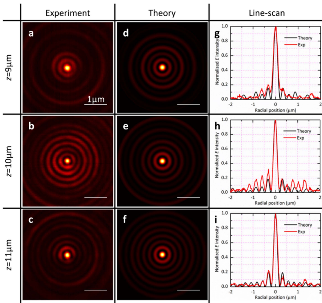
Figure 2 | Transverse electric field intensity profiles. (a–c), Experimentally recorded and (d–f) theoretically calculated diffraction patterns at the propagation distances of z=9 \mu\text{m} (top row), 10 \mu\text{m} (middle row) and 11 \mu\text{m} (bottom row) within the generated optical needle. The contrastive line-scan distributions along the horizontal line across the focal spot center are shown in (g) to (i) respectively.
