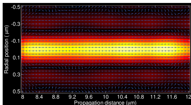
Figure 4 | Normalized Poynting vector distributions in the longitudinal cross-section. In the optical needle region, the Poynting vectors within the mainlobe almost point to the axial direction, indicating the energy flow along propagation. At the super-oscillation regions, the Poynting vectors change their directions rapidly, corresponding to a small amount of energy exchange between the optical needle and the first sidelobes.
