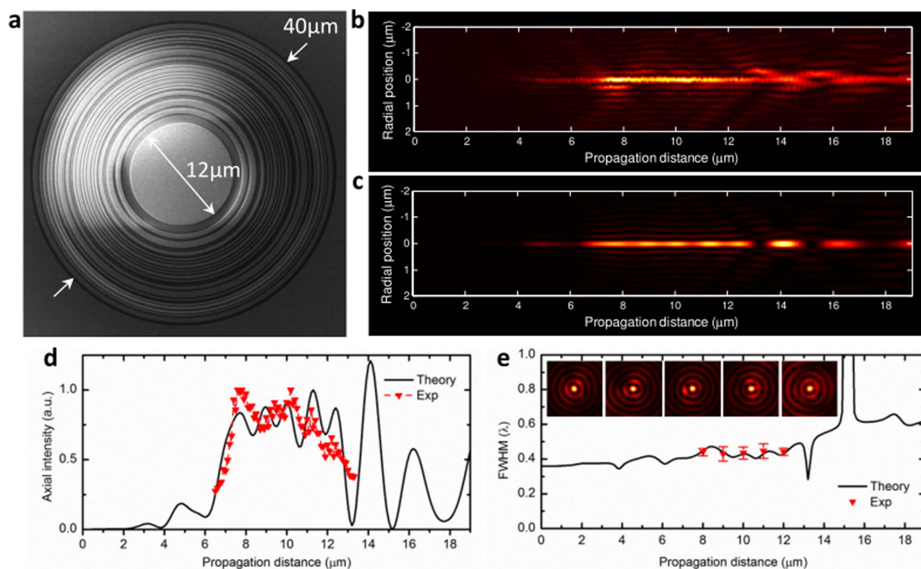
Figure 5 | Central block SOL design for longer DOF. (a), SEM image of Sample 2 which has a central block diameter of 12 \mu\text{m} and is designed with focal length of 10 \mu\text{m} and DOF of 6 \mu\text{m} ; (b), (c), Experimental and simulated intensity of the diffraction patterns within propagation distance of 19 \mu\text{m} respectively; (d), Axial intensity distributions from theory (solid line) and experiment (dashed line with symbol); (e), FWHM of the spot in transverse direction: theory (solid line) and experiment (down triangle). The error bar comes from the spot size averaging along x and y directions. Insets show the transverse intensity distributions within area of 2 \mu\text{m} \times 2 \mu\text{m} at z=8 \mu\text{m} to 12 \mu\text{m} in step of 1 \mu\text{m} .
