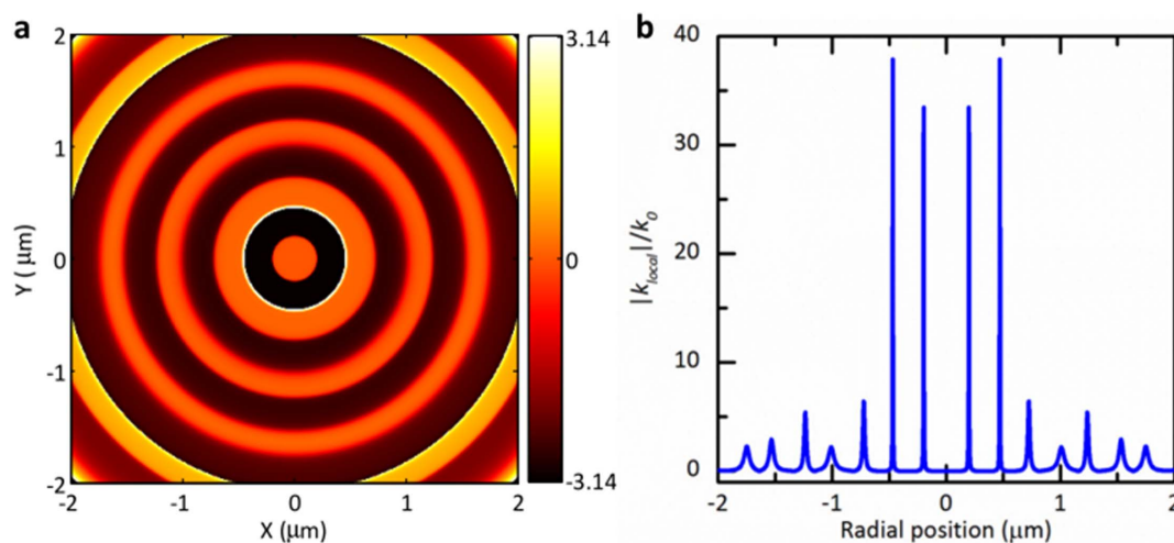
Figure 3 | Phase and local wavevector profiles in focal plane. (a), Phase distributions at z=10 \mu\text{m} , where the central point is used as reference; (b), Local wave-vector distributions along radial direction. The peaks indicate the super-oscillatory regions where k_{\text{local}} is larger than k_0 and the phase oscillates very rapidly.
