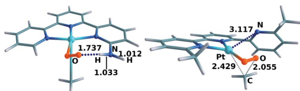
Fig. 9 Optimized geometries of 2\text{-CP}_{(\text{C-}^3\text{C})} (left) and 4\text{-TS}_{(\text{C-G})} (right). Selected distances in \text{\AA} .
