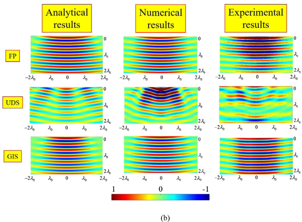
Figure 5. E_z (real part) comparison for all the three samples in terms of analytical, numerical and experimental model along the x-y plane ( \lambda_0 = 30 mm): at (a) 8 GHz and (b) 9 GHz.
