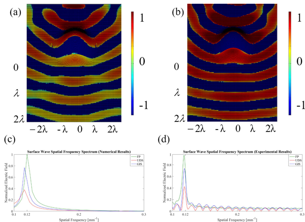
Figure 3. 3D measurements of the E-field on the curved surface for (a) UDS and (b) GIS. Surface Wave Spatial Frequency Spectrum for (c) numerical and (d) experimental results, at 10.0 GHz.
