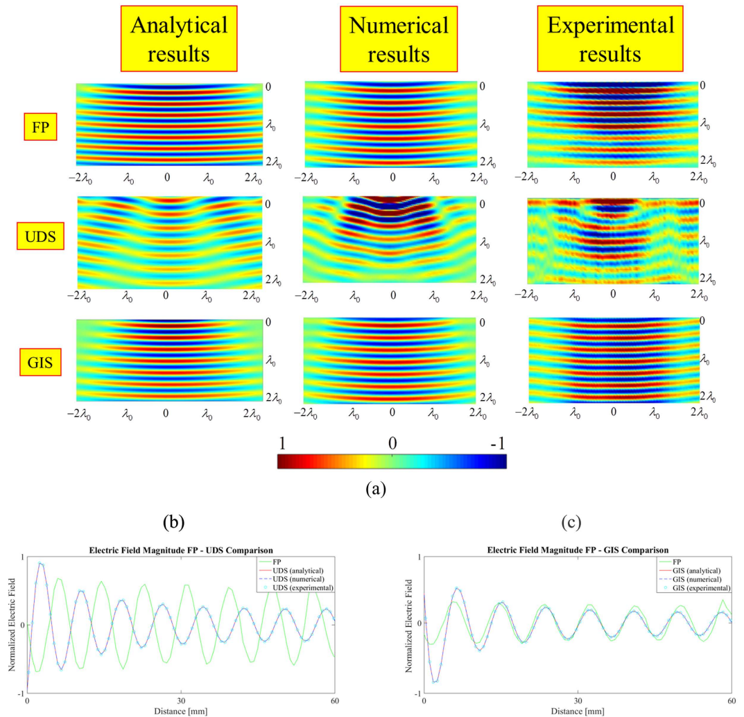
Figure 4. (a) E_z (real part) comparison for all the three samples in terms of analytical, numerical and experimental model along the x-y plane; Magnitude (real part) comparison for the normal electric field E_z (b) FP – UDS and (c) FP –GIS. ( \lambda_0 = 30 mm, f_0 = 10 GHz).
