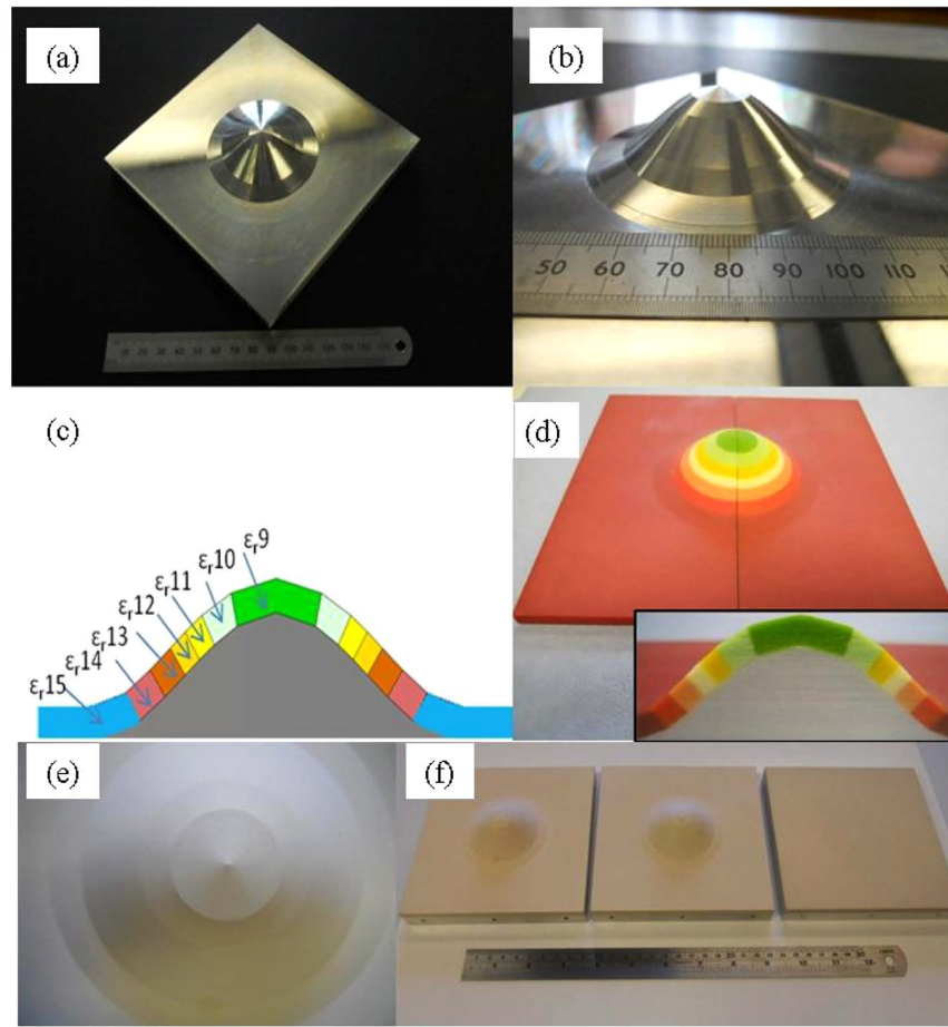
Figure 1. Cosine-shaped surface deformation: (a) top-view and (b) side-view; Schematic indicating the required permittivity values for each layer (c); 3D printed prototype of the cloak structure with cross-section inset (d); Fabricated surface wave structures: (e) plane view of the samples and (f) the three composite structures manufactured.
