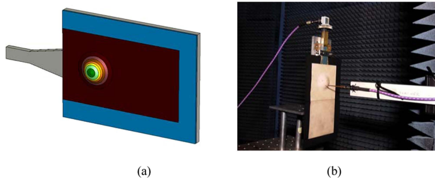
Figure 2. (a) Numerical setup for surface wave cloaking device; (b) Experimental setup for detecting surface waves on devices.
