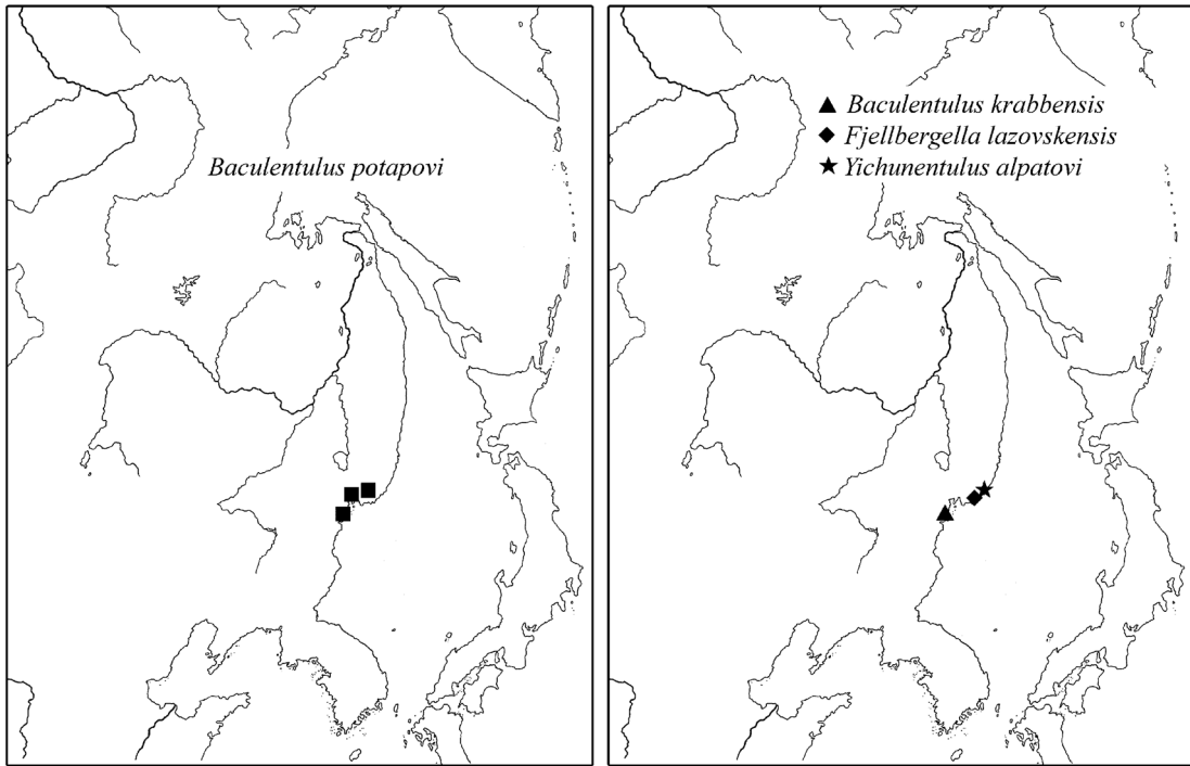
Figure 11. Distribution of some local species of RFE.
