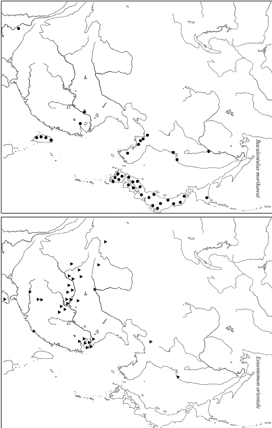
Figure 9. Distribution of two widely distributed East-Asiatic species of RFE. In addition to locations listed in the text, other records are used after Imadaté (1974), Lee and Rim (1988), Szeptycki (2007) and Yin (1999).
