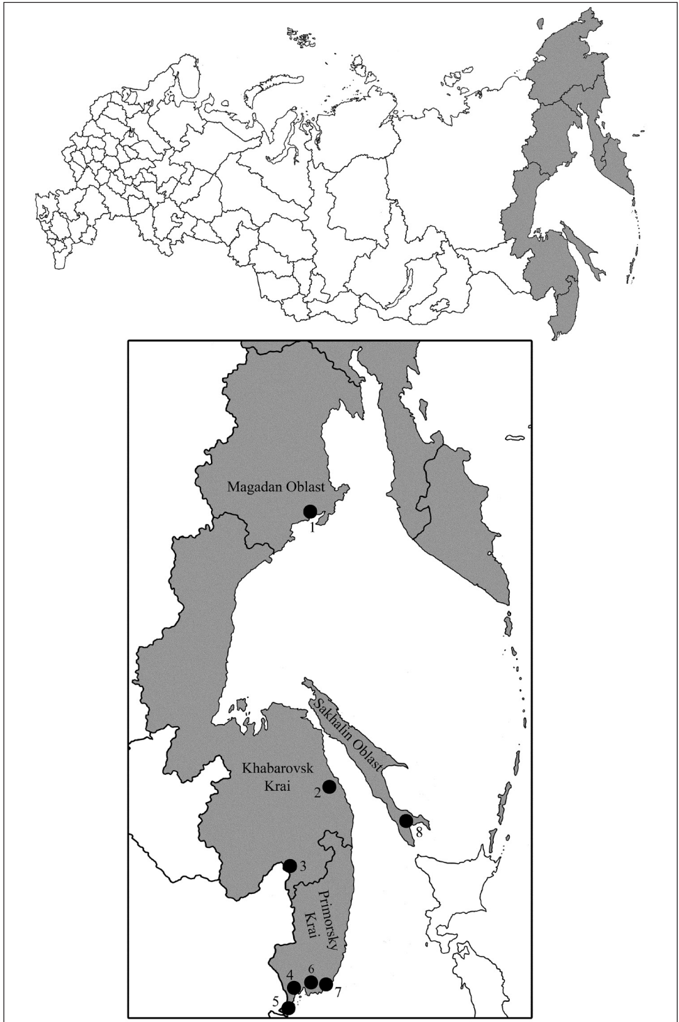
Figure 1. The sampling sites in RFE.
