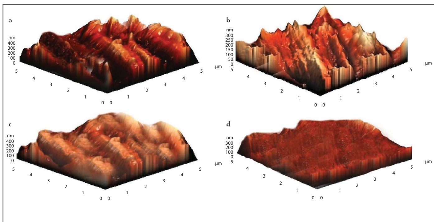
Figure 1. Atomic Force Microscopy imaging of TruNatomy files on exposure to various irrigants (a) On exposure to 5.25% NaOCl for 10 minutes, (b) On exposure to 17% EDTA for 10 minutes, (c) On exposure to combination of 5.25% NaOCl for 8 minutes and 17% EDTA for 2 minutes, (d) No exposure to any irrigant
