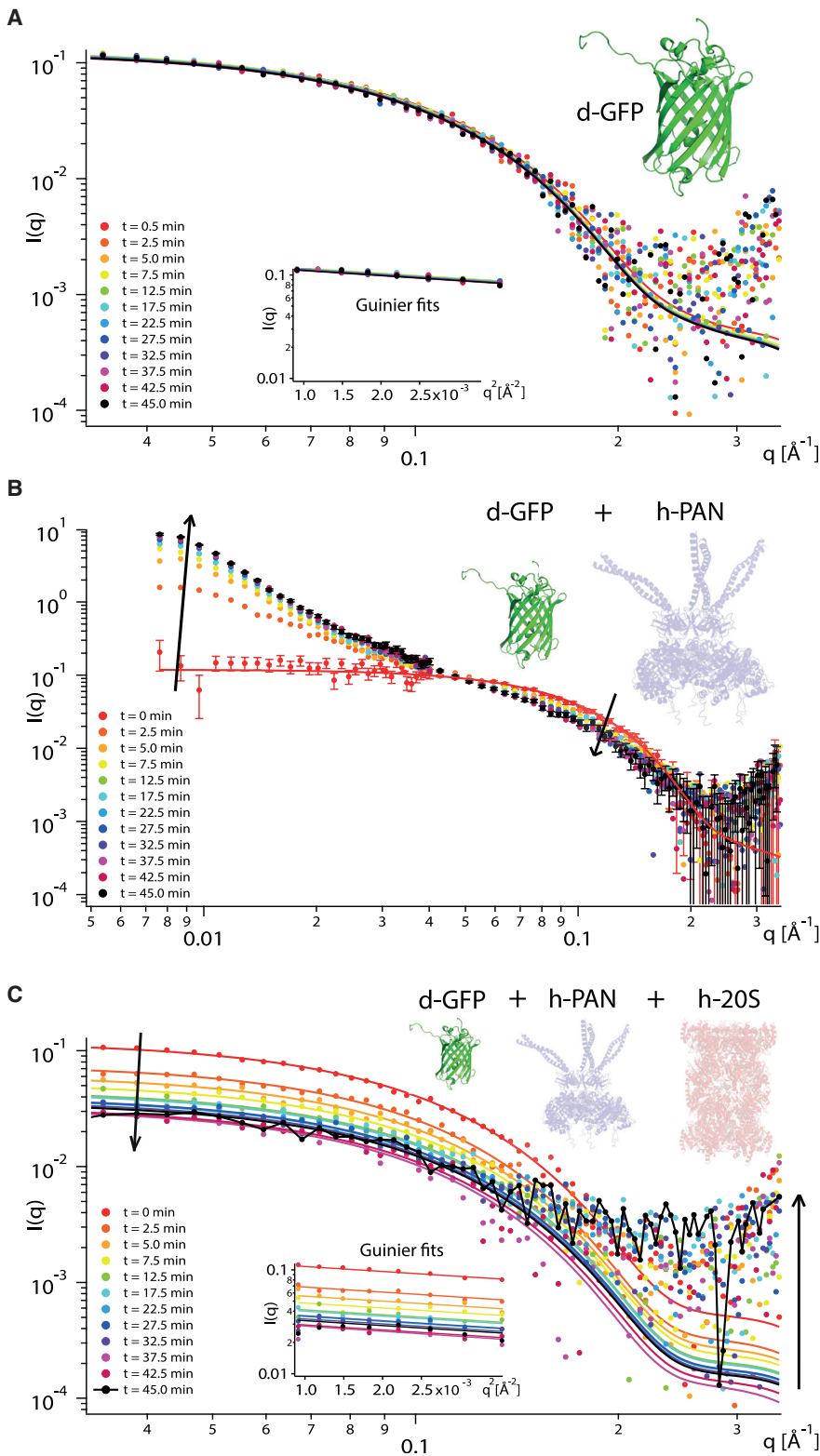
FIGURE 1 Experimental SANS curves as a function of time. Shown are d-GFP alone (A), d-GFP in the presence of h-PAN (B), and d-GFP in the presence of h-PAN and h-20S (C) on a double logarithmic plot. Continuous lines display fits to the atomic Protein Data Bank model with CRYSON (38). Insets in (A) and (C) show the respective Guinier fits used to extract radii of gyration ( R_G ). GFP was perdeuterated in all cases and had a strong contrast in the 42% D_2O (and are therefore depicted as a transparent ribbon ). All samples were measured at 55°C and in the presence of ATP. The arrows indicate the direction of the change of I(q) over time. In (C), the experimental points of the last curve (45 min) are connected by a line to facilitate their visualization at high angles. A total of 90 SANS frames of 30 s were recorded for all samples. For reasons of clarity, only a selection of frames is shown. Likewise, error bars are shown only for the first and last data set in case (B). Typical error bars of the data sets in cases (A) and (C) are shown in Fig. S12. The error bars shown represent statistical errors of the solvent-subtracted SANS intensities as obtained by the program PRIMUS. To see this figure in color, go online.
