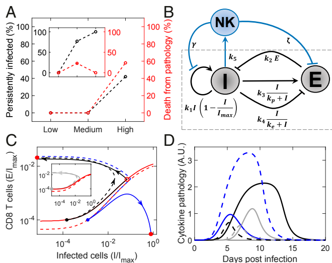
Fig. 3. The influence of NK cells. (A) Outcomes observed experimentally in mice infected with different doses of LCMV clone 13 with ( Inset ) and without NK cells (6). (B) Schematic of the motif embellished to incorporate the influence of NK cells. (C) Projections of trajectories corresponding to low (gray; Inset ), medium- (black), and high-dose (blue) infection with (solid) and without (dashed) NK cells. Projections of the basin boundaries are in red. Three-dimensional versions are in SI Appendix, Fig. S3 . (D) The corresponding time evolution of cytokine pathology. Parameter values are in SI Appendix, Table S1 .
