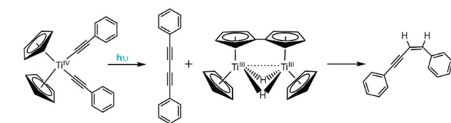
Fig. 8 Irradiation of arylalkynyl titanocene complexes results in photo-induced reductive elimination to form an enyne product.
