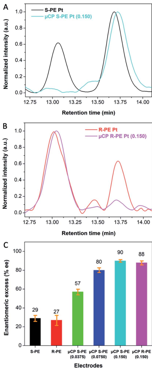
Fig. 3 Characterisation of enantioselectivity; (A) and (B) HPLC chromatograms of the product solutions obtained by electrochemical synthesis performed with (S)-PE and (R)-PE imprinted mesoporous Pt electrodes, respectively, that are either non-coated or coated with thiols by using \mu CP; (C) summary of enantiomeric excess (%ee), obtained after asymmetric electrochemical synthesis carried out with bare (S)-PE (black) and (R)-PE (red) imprinted mesoporous Pt electrodes (0.150 weight ratio PE/PtCl 6 2- ); with (S)-PE imprinted mesoporous Pt electrodes functionalized with thiol ligands by \mu CP, using different (S)-PE/PtCl 6 2- weight ratios in the plating mixture, 0.0375 (green), 0.0750 (dark blue) and 0.150 (light blue); with a (R)-PE imprinted mesoporous Pt electrode obtained from a plating solution with 0.150 weight ratio (R)-PE/PtCl 6 2- and modified with thiol molecules by \mu CP (pink).
