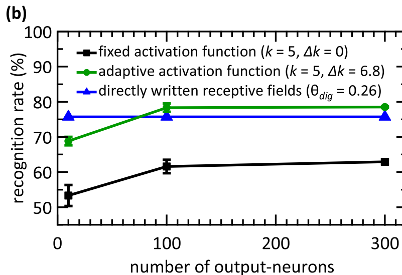
Figure 7. Recognition rates of the StochANN. (a) Shows the combination of the experimental results for MNIST subsets {0, 1, 9} and {0, 3, 8}. Depicted are mean values and standard deviations of five experimental runs for each pattern (i.e. ten runs in total for each data point). The mean value of 100 simulation runs for each pattern set is depicted as dashed line while the standard deviation is depicted as grey area, respectively. Five learning epochs are used in every simulation run. While the abbreviations “poly” and “am” denote the polycrystalline and the amorphous \text{HfO}_{2-x} based devices, “set” and “reset” denote the transition used to emulate stochastic plasticity. In (b) the simulation results for the whole MNIST test set are shown. These results are obtained with a fixed activation function of the output-neurons (black squares) and an adaptive activation function (green circles). The mean values and standard deviations of five runs with five learning epochs are depicted. The direct written receptive fields are shown for comparison (blue triangles). Here, no stochastic mechanisms are involved. Thus, no standard deviation can be denoted. Moreover, an increasing amount of output-neurons does not increase the recognition rate for the latter method, as only one prototype of each pattern can be learned.
