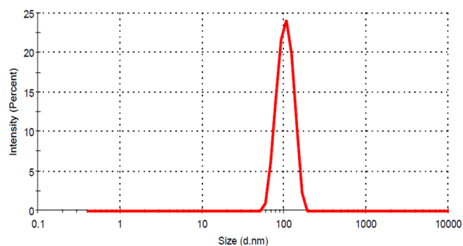
Figure 4. Size determination by hydrodynamic diameter measurement of green synthesized CuO NP nanoparticles by Dynamic light scattering.
