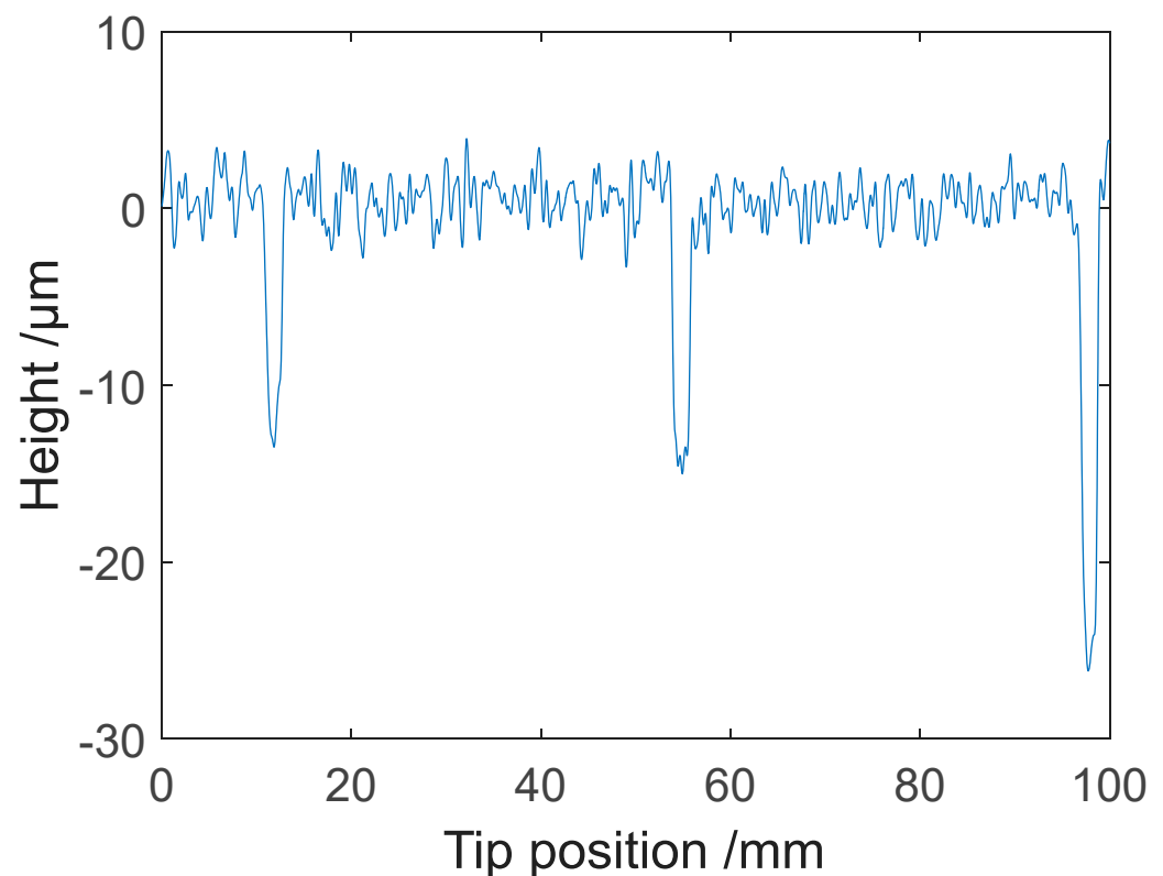
Figure 14. Waviness profile with Gaussian filter and 0.8 mm cut off. Three valleys with depths over 10 \mu\text{m} are visible.
