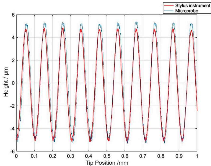
Figure 10. Comparison of the primary profiles of a Mitutoyo 178-601 (S/N 131883) measured with the reference instrument (Talysurf) and with the industrial microprobe setup (at 1.67 mm/s and sampling rate 100 kHz).
