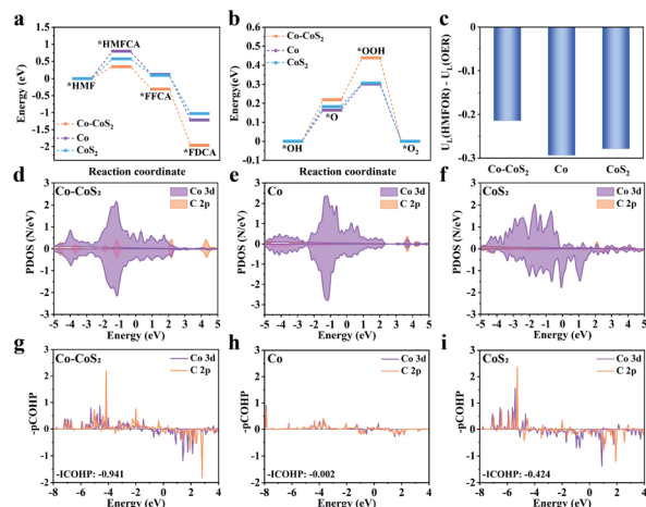
Fig. 5 The free energy diagram of (a) HMFOR, (b) OER, (c) limiting potential ( U_L ) versus [U_L(\text{HMFOR}) - U_L(\text{OER})] , (d–f) PDOS of HMF adsorption, and (g–i) pCOHP and its integrated value (ICOHP) for HMF adsorption on Co-CoS 2 , Co, and CoS 2 .
