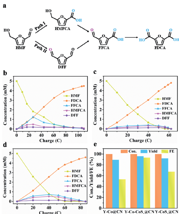
Fig. 4 (a) Two possible reaction pathways for HMF oxidation. The concentration of HMF and its oxidation products in HMF electro-oxidation over (b) Y-Co@CN, (c) Y-Co-CoS x @CN, and (d) Y-CoCoS 2 @CN. (e) HMF conversion, FDCA yield, and FE of Y-Co@CN, Y-Co-CoS x @CN, and Y-CoS 2 @CN in HMF electro-oxidation.
