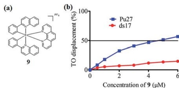
Fig. 2 (a) Chemical structure of complex 9 ; (b) G4-FID titration curves of DNA duplex ds17 and Pu27 G-quadruplex in the presence of increasing concentrations of complex 9 in Tris-HCl buffer. The \text{DC}_{50} value is equal to the half-maximal concentration of compound required to displace 50% TO from DNA.
