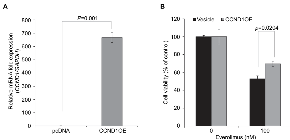
Figure 4 CCND1 overexpression induces everolimus resistance in HSC-I cells.
