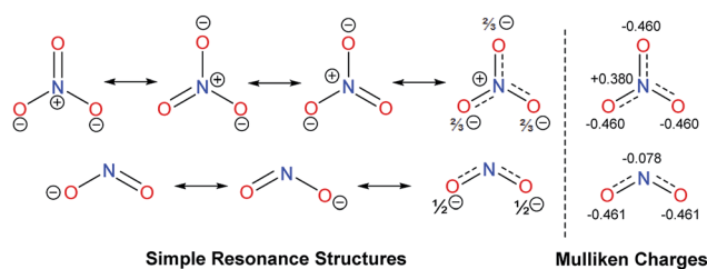
Fig. 4 Resonance structures and calculated Mulliken charges of NO_3^- and NO_2^- anions.
