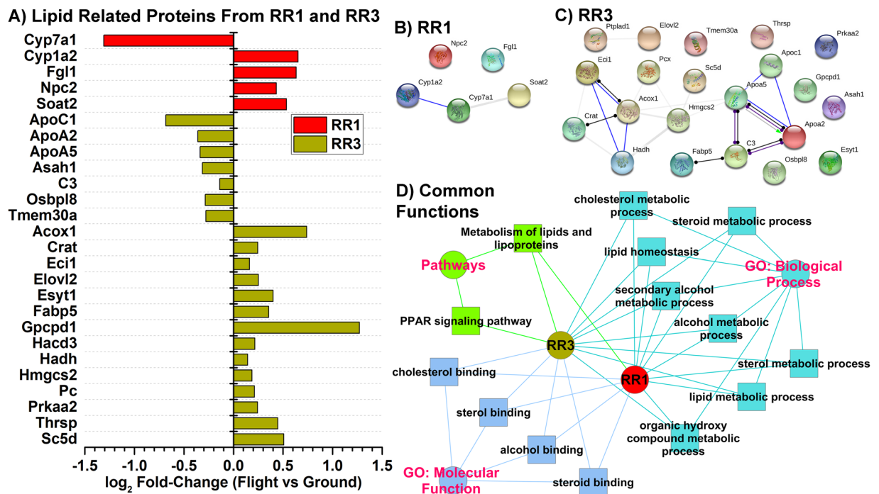
Figure 5. Lipid related proteins from proteomics analysis on livers from mice for RR1 and RR3 datasets. (A) The fold-change ( \log_2 ) values for the lipid related proteins comparing livers from mice from both RR1 and RR3 GeneLab proteomics datasets. (B,C) RR1 and RR3 lipid related protein interaction networks predicted using STRING 41 , which considers both direct (e.g. co-IP) and indirect (e.g. co-expression, text mining) interactions. (D) The overall predicted common Gene Ontology (GO) molecular functions, GO biological processes, and pathways being regulated by all the lipid proteins for both RR1 and RR3 proteomics datasets determined by ToppCluster in the ToppGene Suite 42 . Cytoscape 43 was utilized to displaying the connected network of functions. The colors for the node indicate the group the functions are associated with. The edges (connecting lines between the nodes) represent the connection between either the RR1 or RR3 proteins to the predicted pathways (green line), molecular functions (blue line), or biological process (aqua line).
