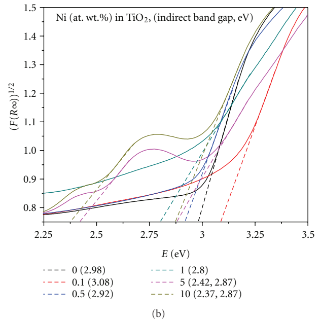
FIGURE 8: Transformed diffuse reflectance spectra of Ni-doped TiO 2 (Ni = 0, 0.1, 0.5, 1, 5, and 10 at. wt.%) powders formed at 550°C for 6 h showing direct bandgap (a) and indirect bandgap (b) energy values.
