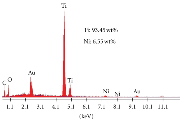
FIGURE 4: EDAX spectra of 5 at. wt.% Ni-doped TiO 2 powder formed at 550°C for 6 h.
