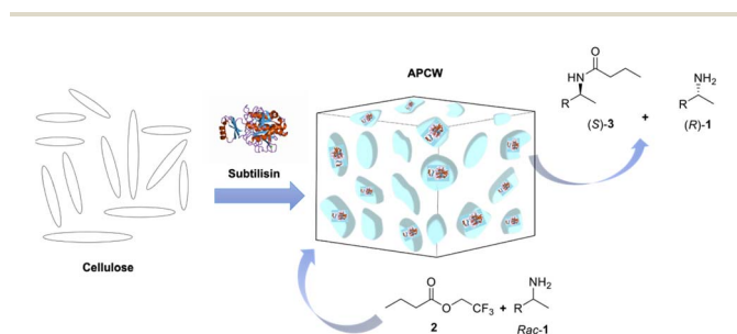
Fig. 1 Simplified scheme of self-assembly of APCW and kinetic resolution of racemic amines 1 .
