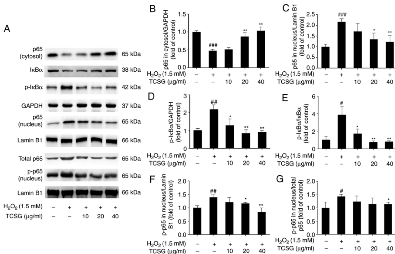
Figure 8. Effect of TCSGs on the activation of the NF- \kappa B signaling pathway in H 2 O 2 -induced L02 cells. Cells were pretreated with the TCSGs (10, 20 and 40 \mu g/ml) for 48 h, and stimulated with H 2 O 2 (1.5 mM) for 24 h. The samples of nuclear and cytosolic proteins were prepared to detect the expression of (A-C) NF- \kappa B p65, (A, D and E) I \kappa B \alpha and p-I \kappa B \alpha , and (A, G and F) p-NF- \kappa B p65 using specific antibodies by western blot analysis, respectively. GAPDH and Lamin B1 were used as the internal controls. All results are presented as the means \pm standard deviation (n=3). *P<0.05, **P<0.01 and ***P<0.001 vs. the control group (no treatment); #P<0.05 and ##P<0.01 vs. H 2 O 2 group. TCSGs, total C-21 steroidal glycosides; H 2 O 2 , hydrogen peroxide; NF- \kappa B, nuclear factor- \kappa B; I \kappa B \alpha , inhibitor of nuclear factor- \kappa B; p-, phosphorylated.
