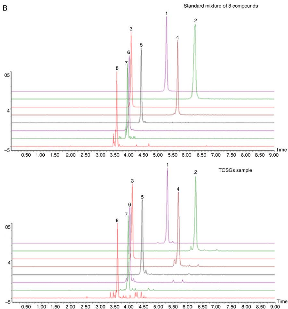
Figure 1. Continued. (B) The total ion chromatograms of 8 standard compounds and TCSGs by multiple reaction monitoring. No. 1, caudatin-2,6-dideoxy-3-O-methyl- \beta -D-cymaropyranoside; no. 2, wilfoside C1N; no. 3, caudatin; no. 4, wilfoside K1N; no. 5, wilfoside C1G; no. 6, cynauricoside A; no. 7, cynauricoside C; no. 8, auriculoside IV. TCSGs, total C-21 steroidal glycosides.
