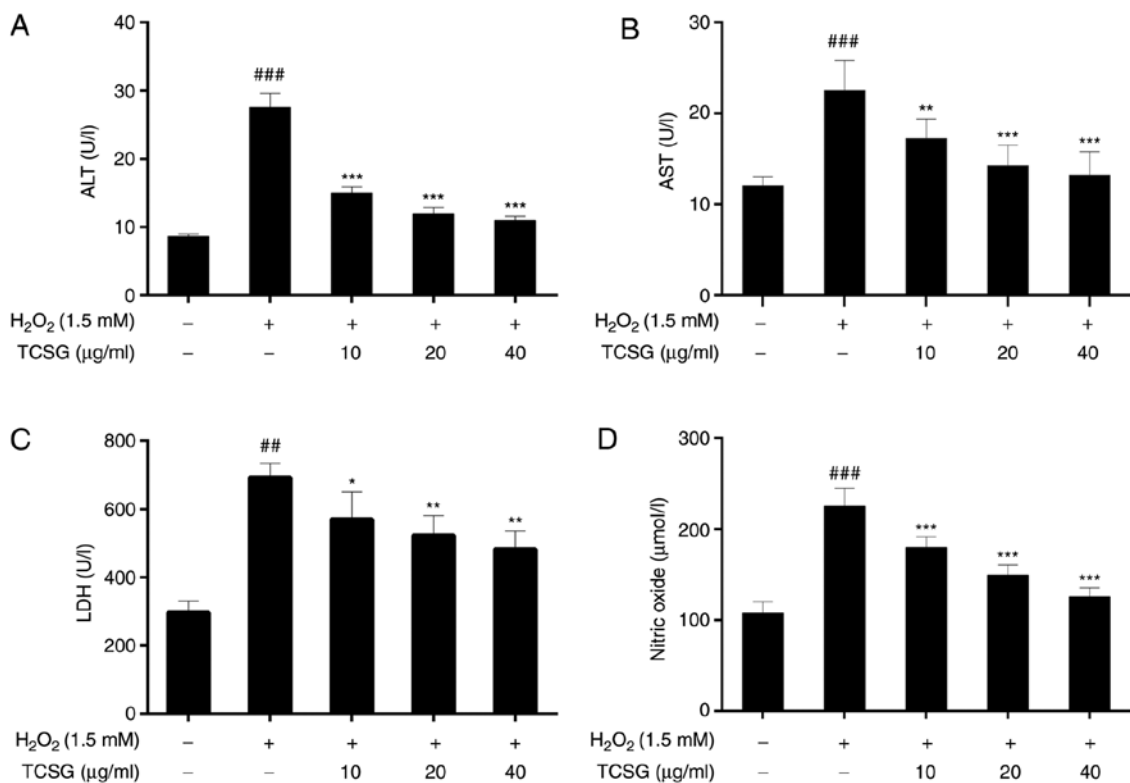
Figure 3. Effect of TCSGs on the supernatant levels of (A) ALT, (B) AST, (C) LDH and (D) NO in H_2O_2 -exposed L02 cells. Data are expressed as the means \pm standard deviation ( n=5 ). \#\#\#P<0.001 vs. the control group (no treatment); \#P<0.05 , \#\#\#P<0.001 vs. H_2O_2 group. TCSGs, total C-21 steroidal glycosides; H_2O_2 , hydrogen peroxide; ALT, alanine aminotransferase; AST, aspartate aminotransferase; LDH, lactate dehydrogenase; NO, nitric oxide.
