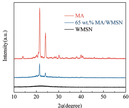
Fig. 4 XRD diffraction patterns of MA, WMSN and 65 wt% MA/WMSN composite.
