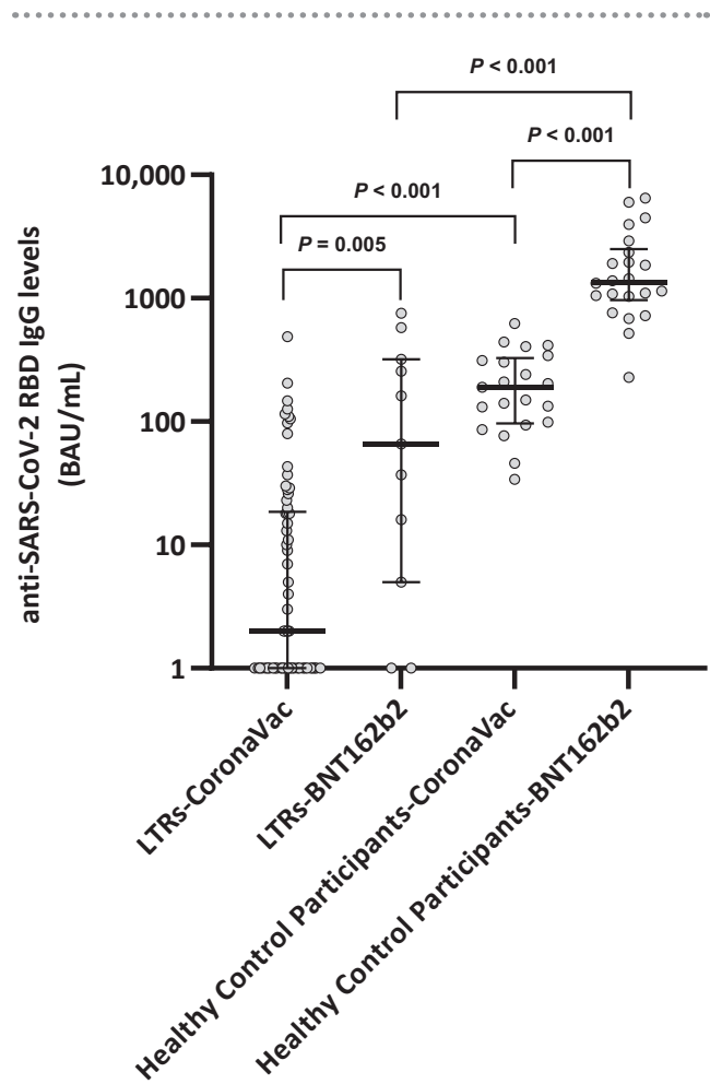
FIG. 1. Specific anti-RBD SARS-CoV-2 IgG levels in LTRs and healthy control participants fully vaccinated with 2 doses of either the BNT162b2 or CoronaVac vaccines. IgG levels are expressed in BAU/mL, by using the WHO International Standard for anti-SARS-CoV-2 immunoglobulin (NIBSC code 20/136) for assay calibration. Medians and IQRs are indicated by horizontal bars. Differences between independent-group continuous data were analyzed by Mann-Whitney U test.
