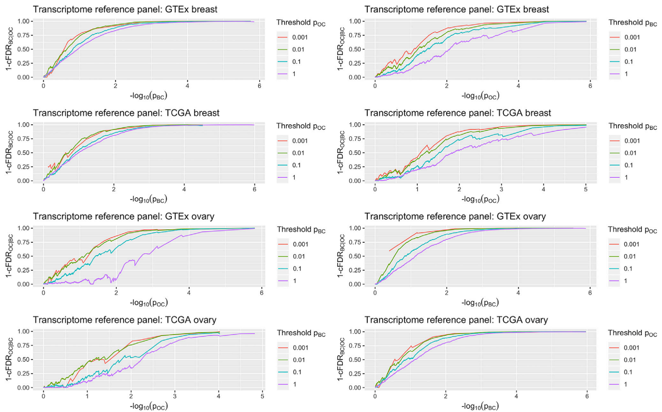
Figure 2. True discovery rate of S-PrediXcan associations for each cancer stratified by associations with the other cancer
