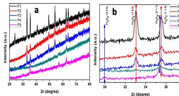
Fig. 1 Full XRD patterns (a) and magnified XRD pattern (b) of the \alpha - \text{Fe}_2\text{O}_3/\text{Fe}_3\text{O}_4 prepared using different water to EG ratios as a solvent.
