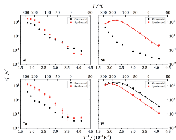
Fig. 12 {}^7\text{Li} NMR relaxation rates T_1^{-1} vs. inverse temperature for commercial and synthesized Al-, Nb-, Ta-, and W-substituted LLZO. Solid lines show fits according to eqn (1) and (2).
