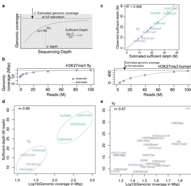
Figure 3. Estimation of fully saturated genomic coverage and sufficient depth. (a) Diagram of how fully saturated genomic coverage and sufficient depth were estimated. (b) Example of observed and estimated genomic coverage for H3K27me3 in fly (left) and human (right). (c) Comparison between the estimated sufficient depth using the model and the observed sufficient depth calculated from the full data in Figure 2b. (d) Estimated genomic coverage at full saturation and sufficient depth. Human H3K9me3 was not included because 55 million reads were insufficient for this estimation. (e) Predicted genomic coverage at full saturation and sufficient depths for 22 fly marks in late embryos. Marks in blue indicate results from the deep-sequenced data, as in panel (c).
