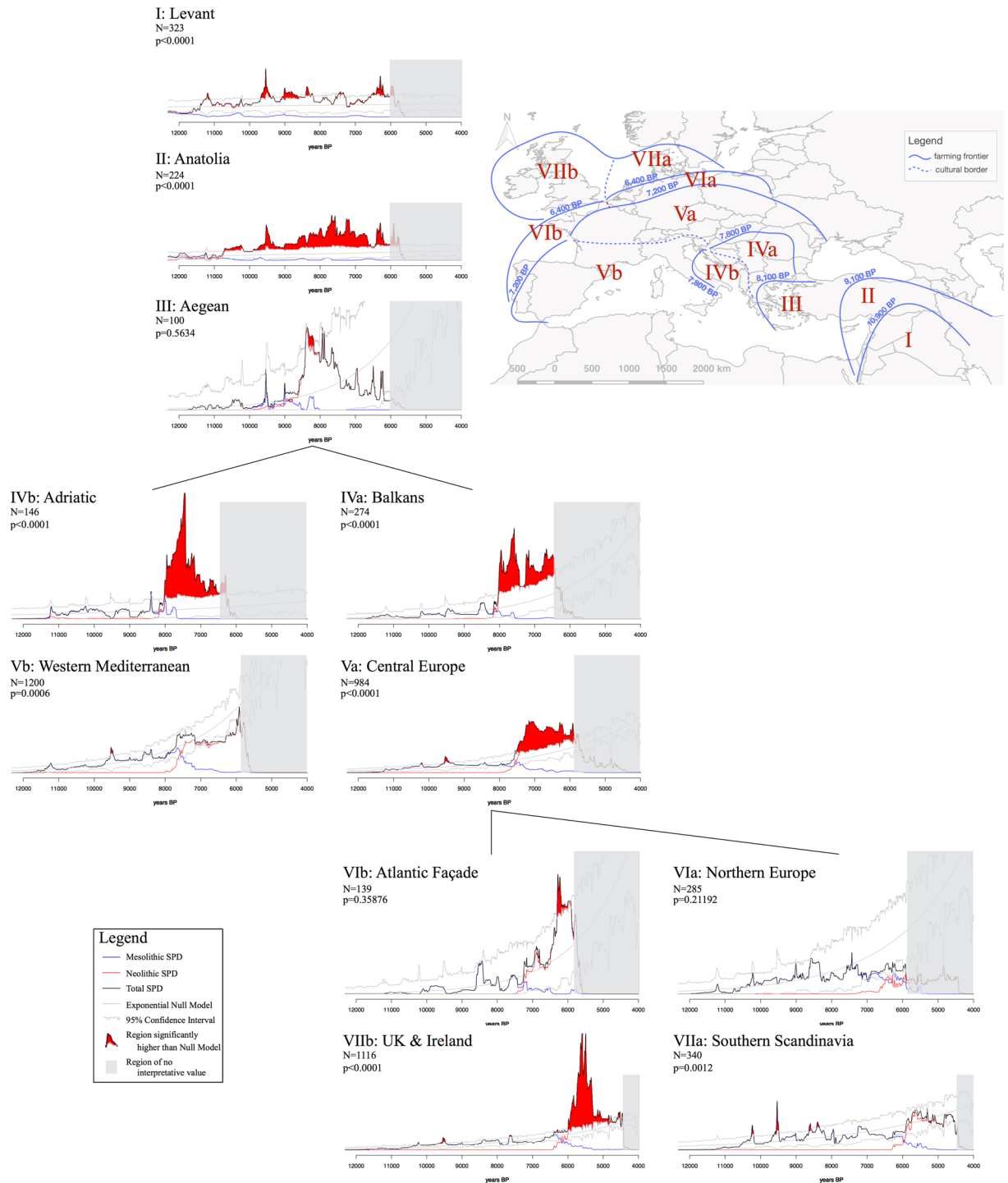
Figure 4. Sum of Radiocarbon Probability Densities (SPD) for each region. The regions are identified in the map at the top-right. SPDs for the local Mesolithic (blue line) and Neolithic (red line) subsets are shown, as is the fitted null model of exponential growth (grey line) and its 95% confidence interval. Values above this confidence interval are highlighted in red. Sub-sampled time periods, corresponding to the end of the sampling range, hold no interpretative value and are, therefore, covered in grey shading. Map generated with QGIS version 2.14.3-Essen ( www.qgis.org ) and other figures generated with R version 3.3.2 ( www.r-project.org ).
