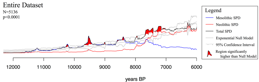
Figure 3. Sum of Radiocarbon Probability Densities (SPD) for the entire dataset (black line). SPDs for the Mesolithic (blue line) and Neolithic (red line) subsets are also shown, as is the fitted null model of exponential growth (grey line) and its 95% confidence interval. Values above this confidence interval are highlighted in red. Figure generated with R version 3.3.2 ( www.r-project.org ).
