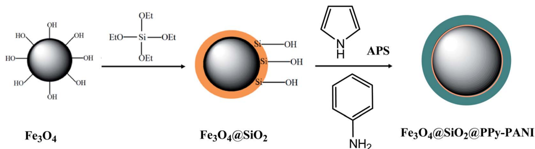
Fig. 1 A schematic diagram for the synthesis of \text{Fe}_3\text{O}_4@SiO_2@PPy-PANI magnetic nanocomposite.
