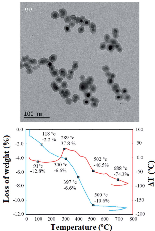
Fig. 2 (a) The TEM image and (b) the TG plot of the \text{Fe}_3\text{O}_4@SiO_2@PPy -PANI magnetic nanocomposite.
