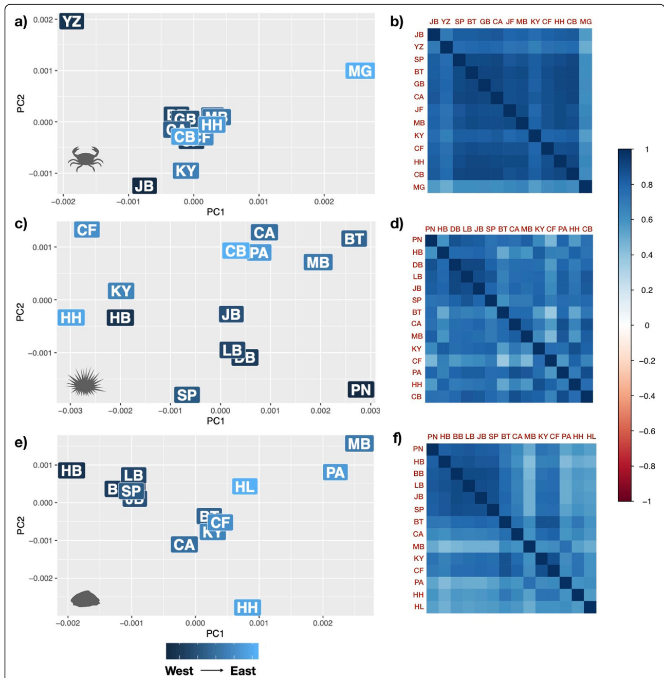
Fig. 2 Population differentiation is shown by PCoAs of Nei's genetic distance from all quality-filtered SNPs (a, c, e) and covariance ( \Omega ) matrices represented as heatmaps (b, d, f), shown for C. punctatus (a, b), P. angulosus (c, d), and S. granularis (e, f). Letters in the PCoAs (a, c, e) correspond to the sample sites shown in Fig. 1, with darker shaded letters corresponding to western sites, and lighter shaded letters corresponding to eastern sites
