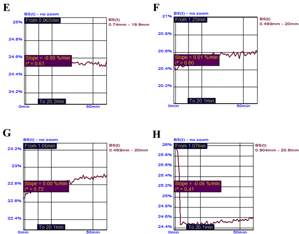
Fig. (3). Kinetic profile of backscattering ( \Delta BS) for Iloprost solution-loaded DIPs. The slope of \Delta BS was evaluated at different incubation times: (E) day 5; (F) day 6; (G) day 7; (H) day 8. 20 mm of samples were analyzed for 1 h at room temperature. Results are the average of three different measurements \pm standard deviation.
